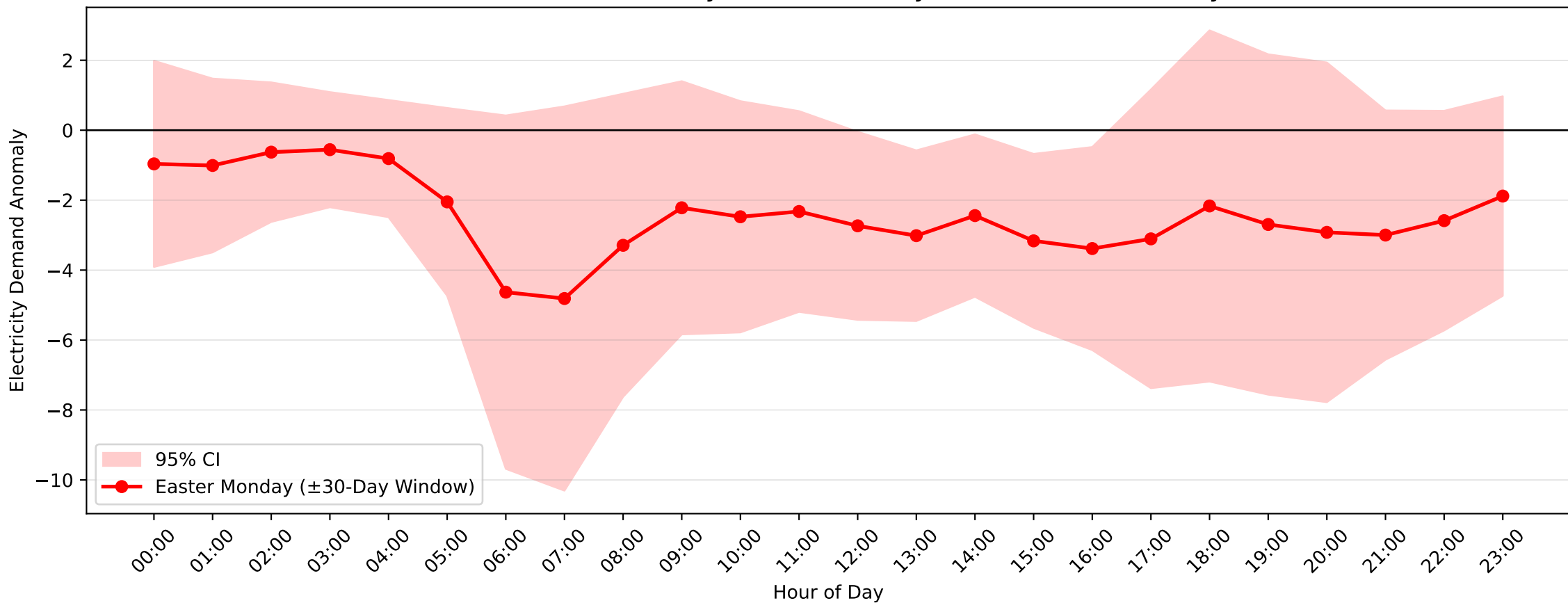
Pennant Hills Demand Anomaly: Easter Monday (2004–2017, \pm 30 -Day Window)
